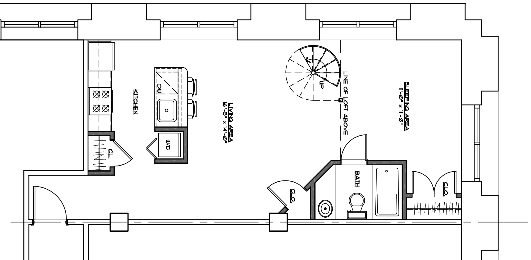
LOWER LEVEL PLAN (UNIT 101A) SCALE 3/16"=1'-0"
